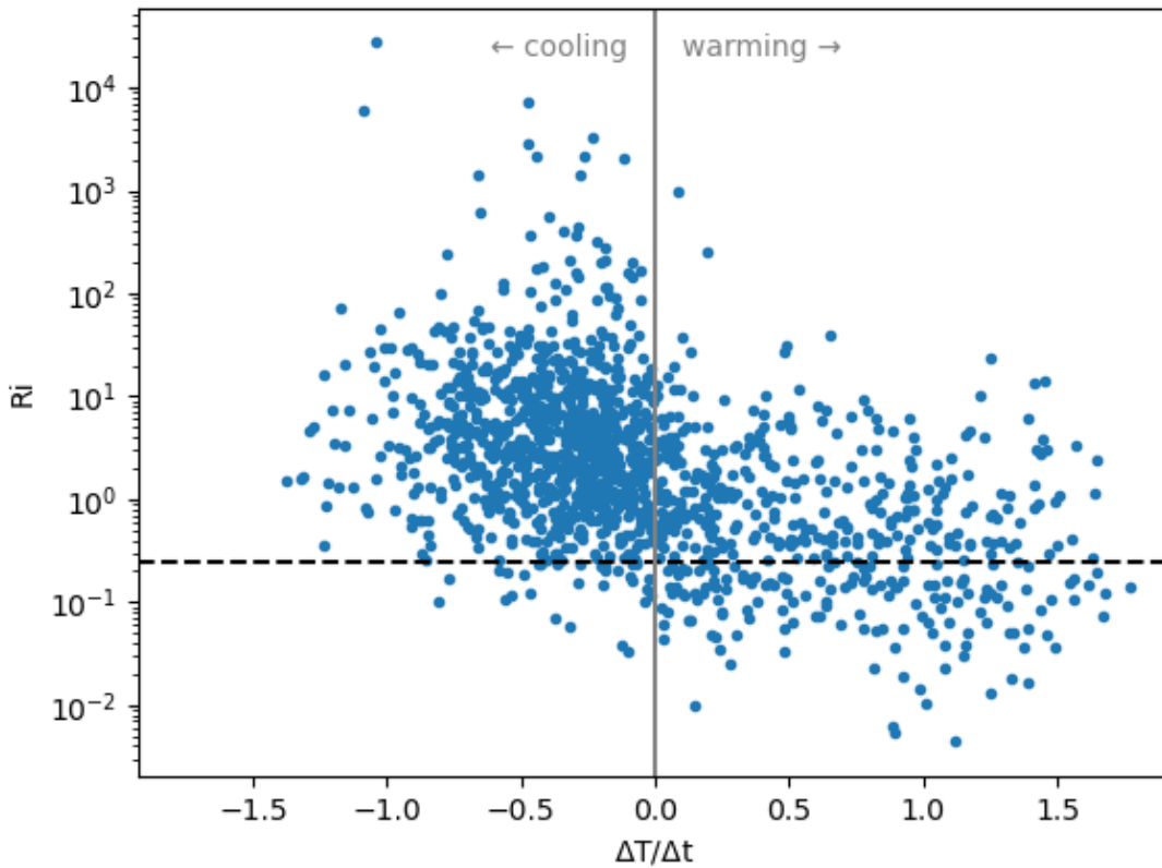
Figure 6. Values of the gradient Richardson number, Ri , compared with the change in temperature over time, \Delta T/\Delta t (units of ^{\circ}\text{C per hour} ). The horizontal black dashed line indicates Ri = 0.25 . Values below this line indicate conditions favorable for shear-driven turbulence. The vertical gray line indicates \Delta T/\Delta t = 0 at 1.6 mab. Higher values indicate that the water is warming over time, while lower values indicate that the water is cooling over time.
